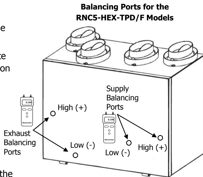
Digital manometer connection overview
