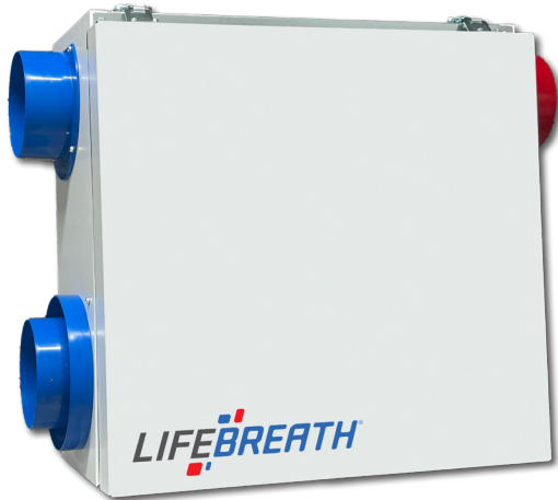
METRO 120 ERV-ECM 117 CFM @ 0.3 (75) IN. W.G. (PA)
